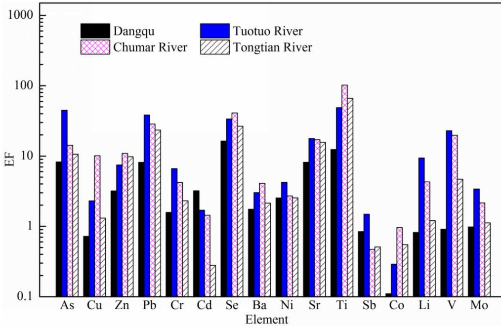
Figure 4 | Enrichment factor of trace elements in different rivers in the SRYS.
